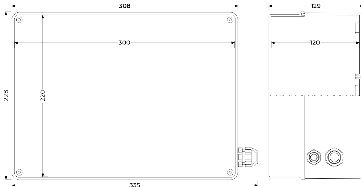
General view of the device
