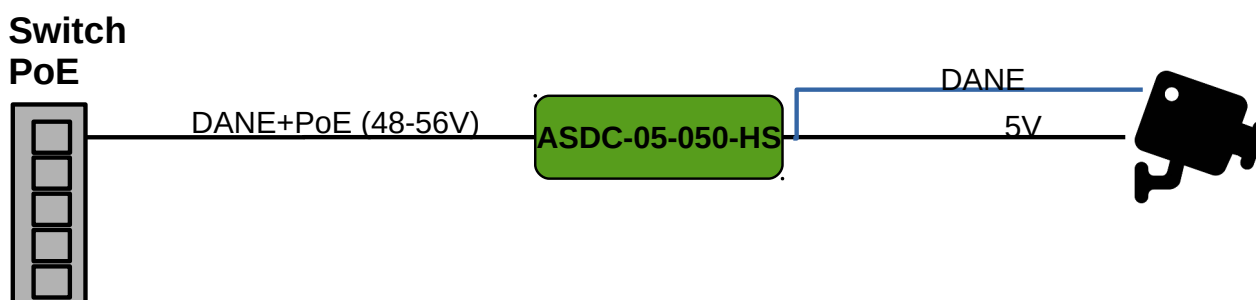
Typical application
